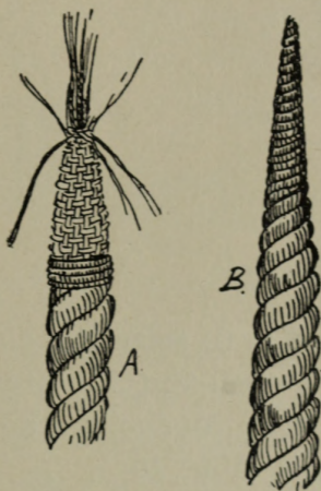
FIG. 103.—Pointing a rope.
